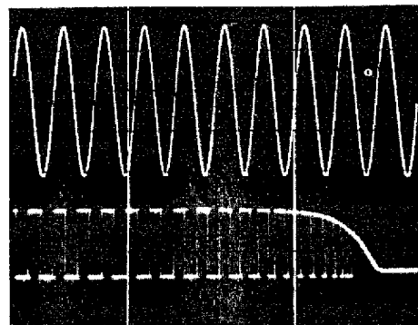
Figure 3. Two cursors may be positioned by the user or controller, at points of interest on either waveform. The voltage difference, time difference, or 1/time difference, as well as the absolute values may be directly read from the LED display, or sent to a controller. Positioning may be precisely accomplished with the aid of the "zoom" feature.
